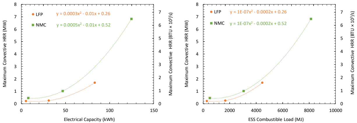
Figure 7-5: Maximum convective HRR energy as a function of electrical capacity and combustible load for the LFP and NMC tests.
