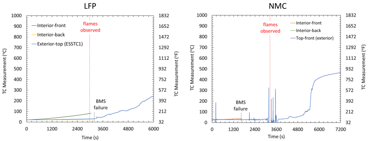
Figure C-2: TC measurements from module BMS for LFP (left) and NMC (right).
