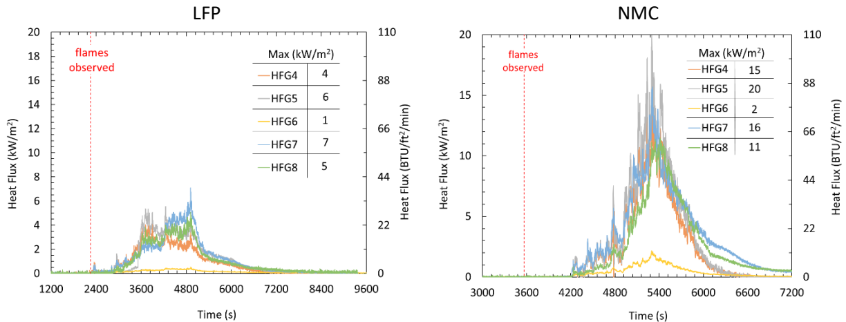
Figure 6-11: Thermal exposure to surroundings during LFP (left) and NMC (right) test. HFG4-5 & 7-8 were near-field measurements at 2.7 m (9 ft) horizontally from the closest edge of the ESS; HFG6 was a far-field measurement at 11.6 m (38 ft).
