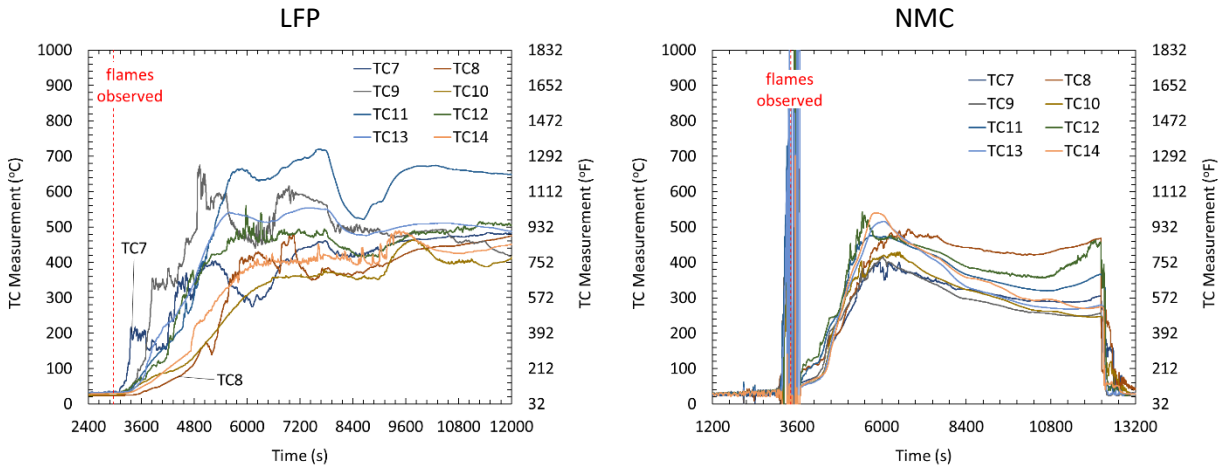
Figure C-3: TC measurements from the mock modules in the LFP (left) and NMC (right) tests.
