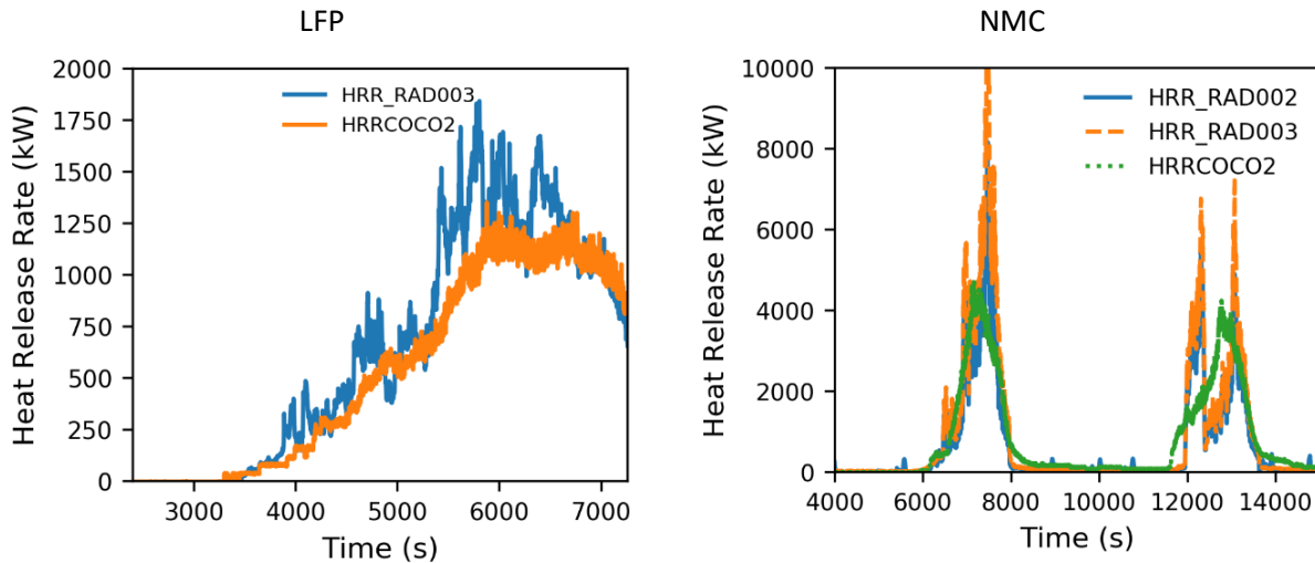
Figure 3-9: Chemical heat release rates calculated based on CO/CO 2 calorimetry and radiation measurement, sprinklered LFP test (left) and sprinklered NMC test (right).
