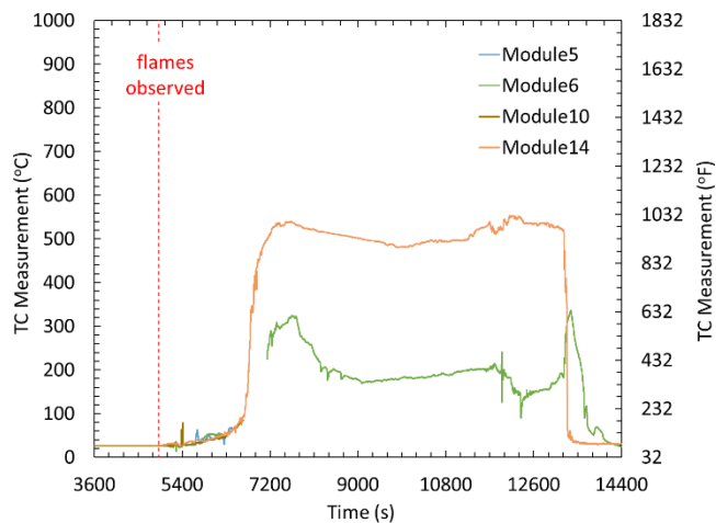
Figure 3-7: Example of edited TC measurements during the sprinklered NMC Test. Module14 included as an example of a data series that did not require editing.
