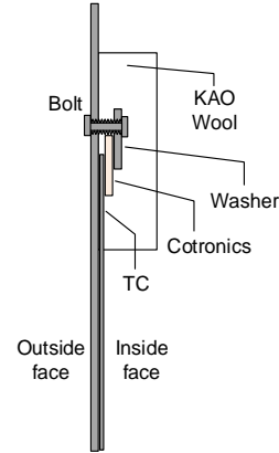
Figure 3-8: Photo of backside of TCs installed on mock ESS rack (TC28 – 37) on left and schematic of TC attachment on right.
