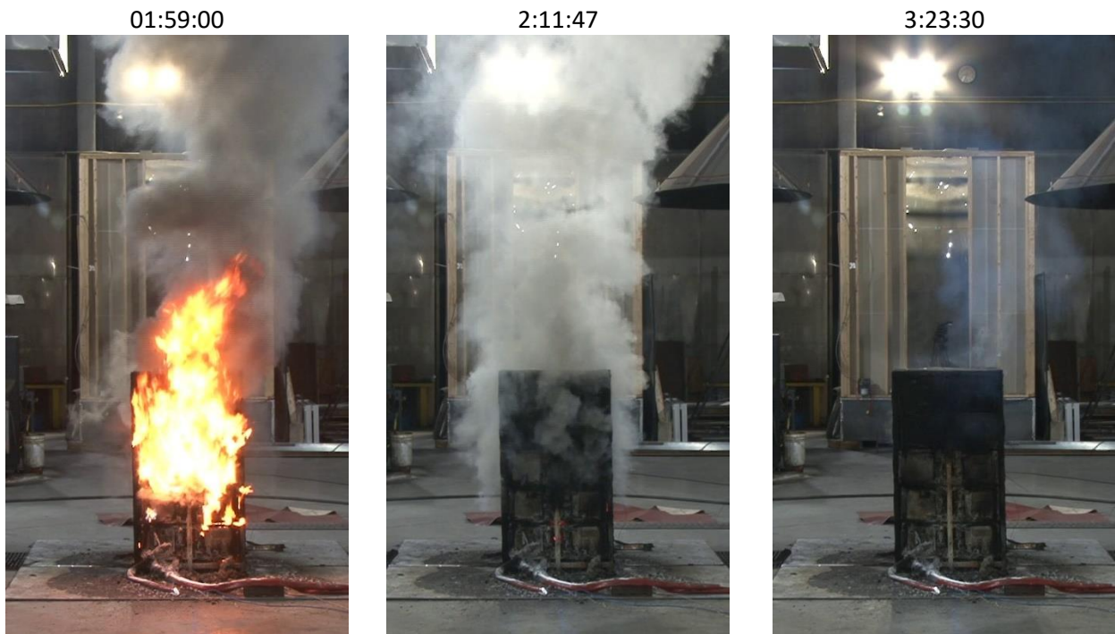
Figure 5-6: Photos of NMC fire decay phase (left), at burn-out of all modules (middle), and post-test (right).
