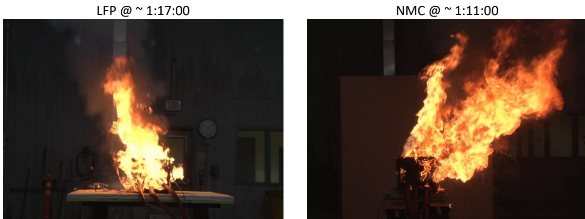
Figure 4-8: Photos of LFP (left) and NMC (right) at near peak heat release rate. The angle of the flames is due to the momentum of the vent gases exiting the batteries.
