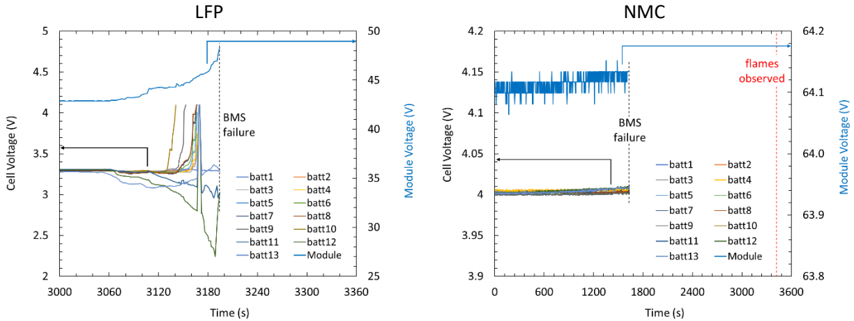
Figure C-1: Voltage measurements from module BMS for LFP (left) and NMC (right) tests.
