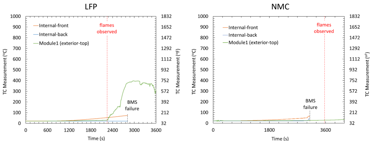
Figure D-2: TC measurements from module BMS for LFP (left) and NMC (right)
