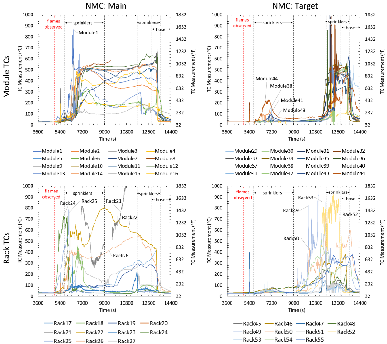
Figure 6-26: TC measurements during NMC test for main (left) and target (right) racks: module temperatures (top), rack temperatures (bottom).
