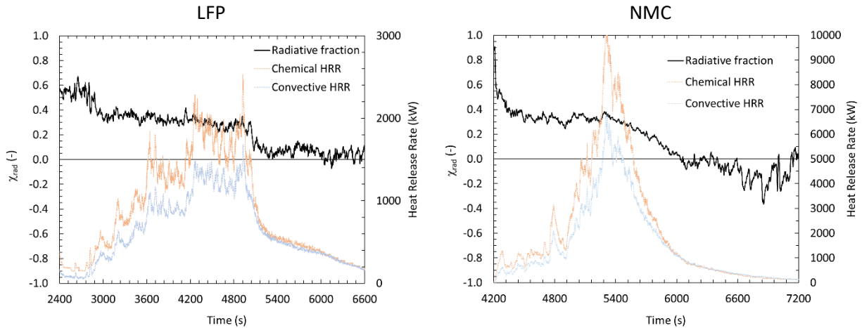
Figure 6-16: Radiant fraction based on convective and chemical heat release rate measurements for the LFP (left) and NMC (right) tests.
