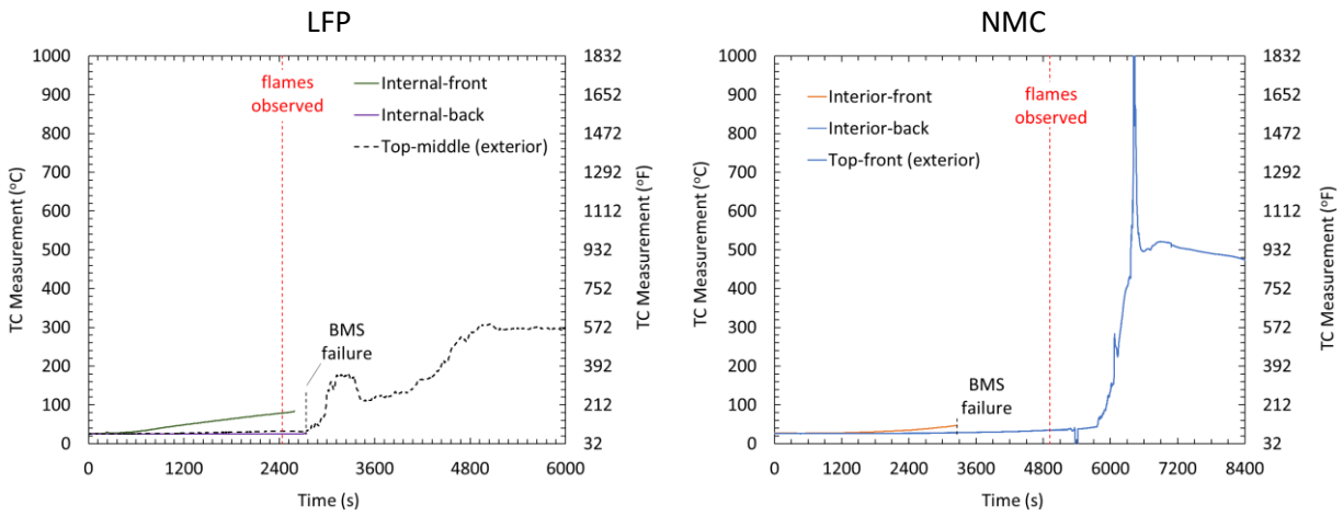
Figure D-4: TC measurements from module BMS for LFP (left) and NMC (right)
