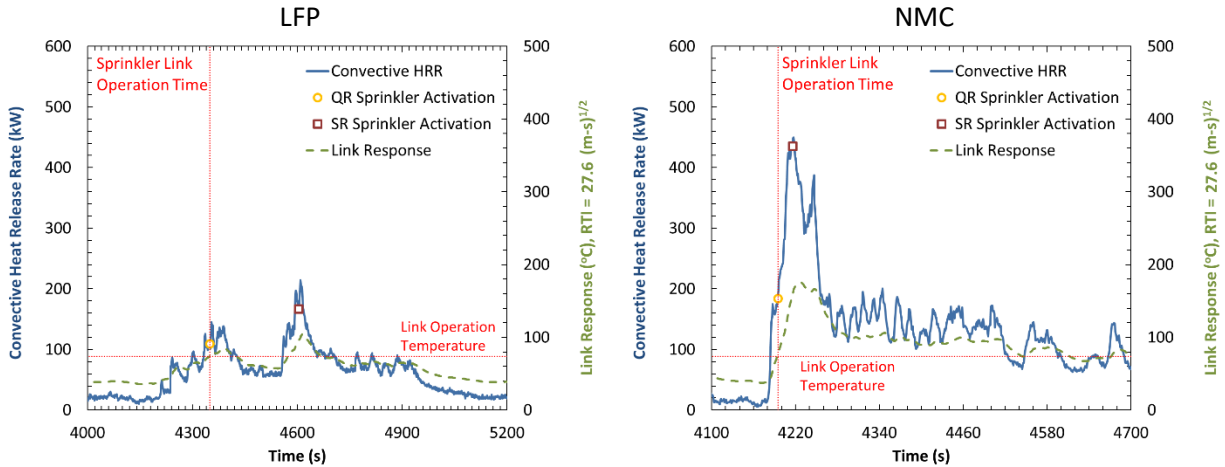
Figure 4-13: Predicted sprinkler response during LFP (left) and NMC (right) free burn test. Dashed green line shows the response of a QR link installed under a 4.6 m (15 ft) ceiling, directly over the fire.
