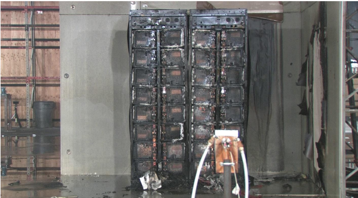
Figure 6-24: Post-test photo of NMC showing complete burnout of main and target rack.
