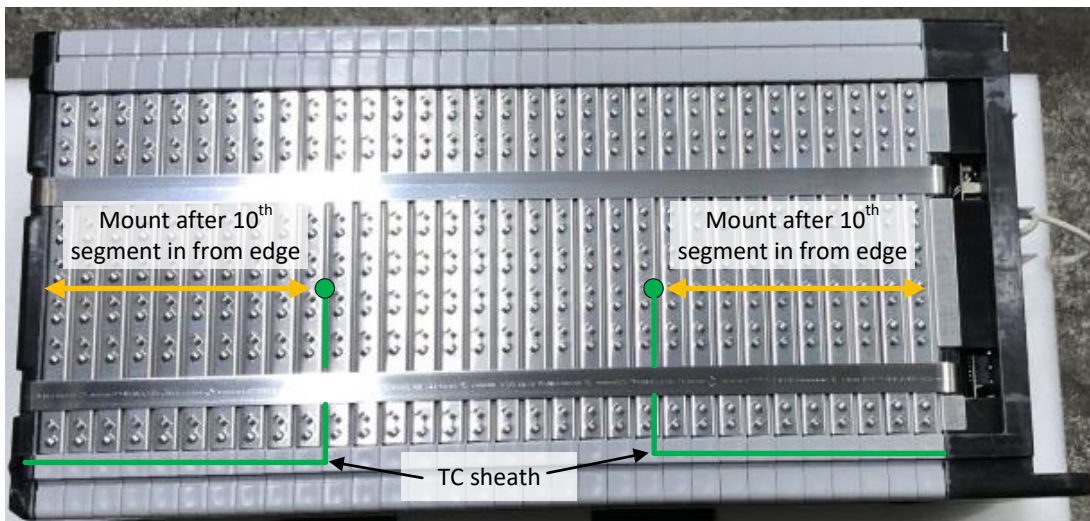
Figure 4-3: Thermocouple layout, NMC
