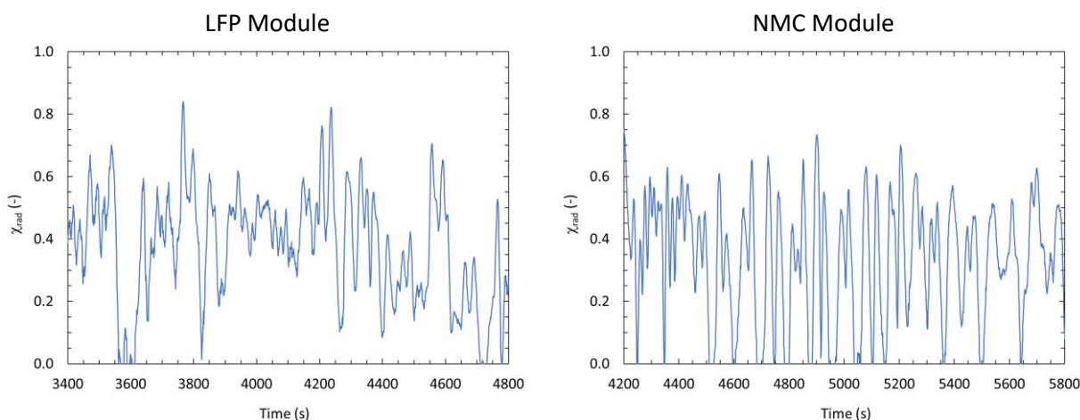
Figure 4-12: Radiative fraction based on convective and chemical heat release rate calculations; LFP (left) and NMC (right). Data shown as a 10-s average.
