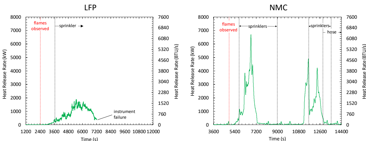
Figure 6-28: HRR for LFP (left) and NMC (right) based on far-field radiation measurements in the sprinklered test environment.
