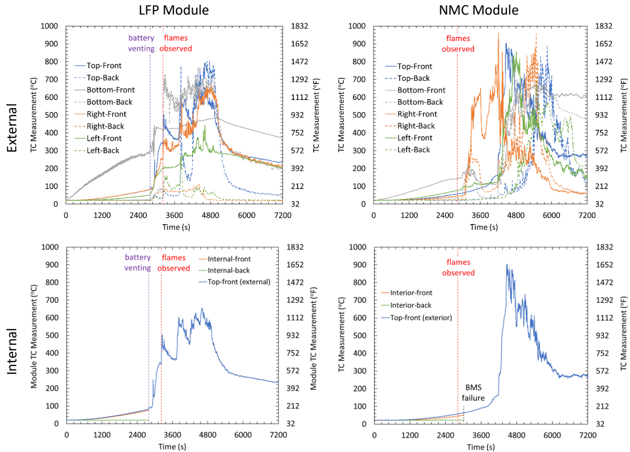
Figure 4-9: TC Measurements on the exterior and interior of the modules; LFP (left) and NMC (right)
