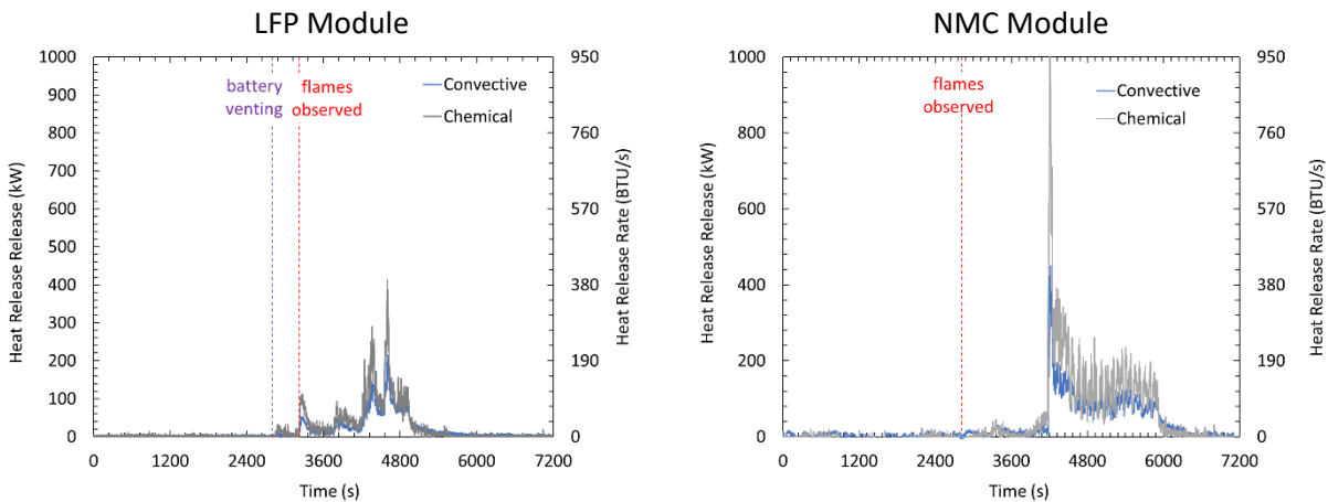
Figure 4-11: Heat Release Rate; LFP (left) and NMC (right).
