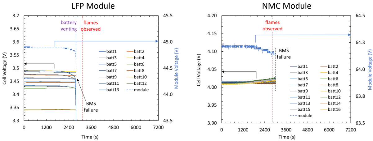
Figure 4-10: Voltage response from BMS for LFP (left) and NMC (right) tests.
