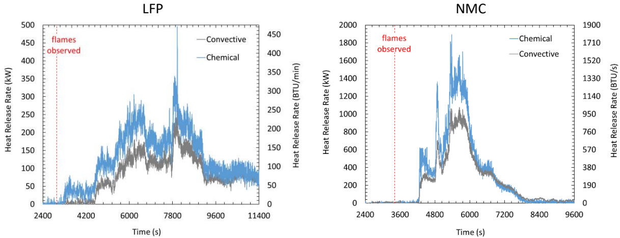
Figure 5-9: Heat Release Rate; LFP (left) and NMC (right).
