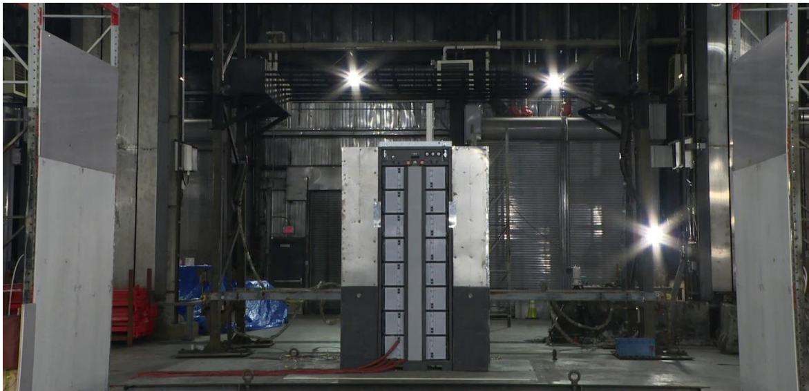
Figure 6-1: Example of full-scale free burn test setup for the NMC module. Mock racks are located on either side of the ESS rack to measure the exposure hazard to adjacent equipment and representative structure walls are located across a 2.7-m (9-ft) separation to measure the exposure to surrounding objects.
