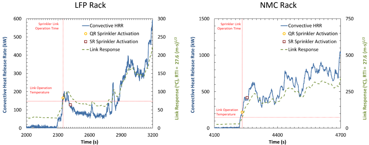
Figure 6-17: Predicted sprinkler response during LFP (left) and NMC (right) free burn test. Dashed green line shows the response of a QR link installed under a 4.6 m (15 ft) ceiling, directly over the fire.
