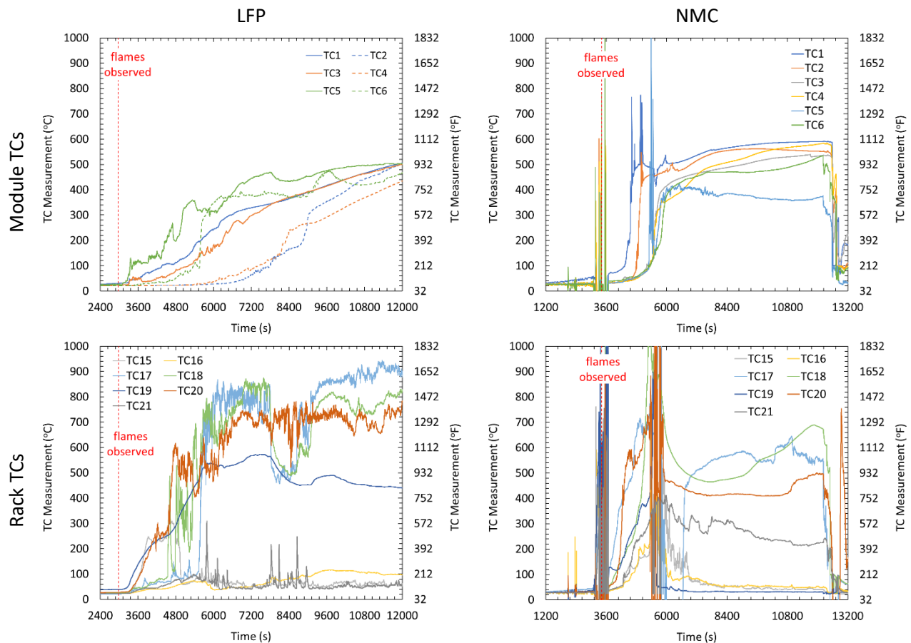
Figure 5-7: TC measurements during LFP (left) and NMC (right) tests for modules (top) and target (bottom).
