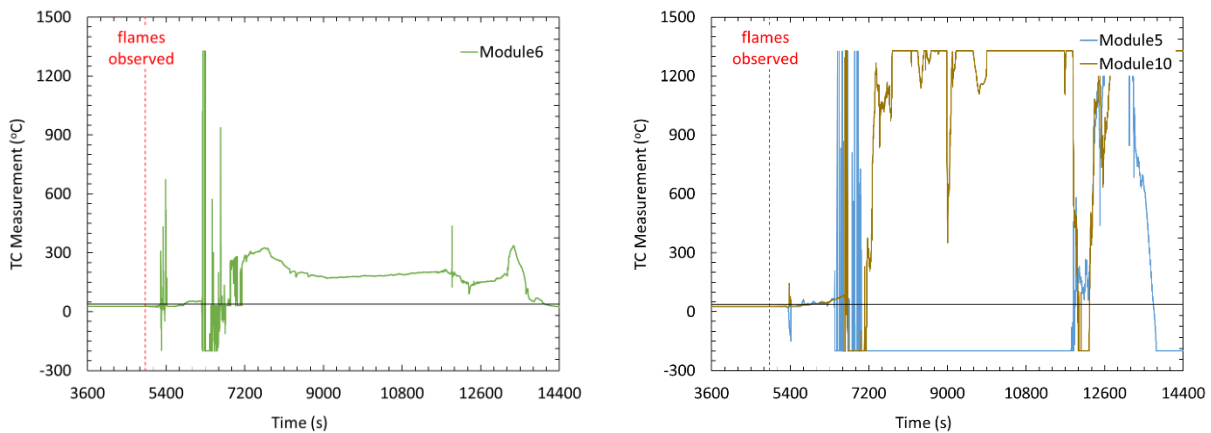
Figure 3-6: Example of original TC Measurements during the sprinklered NMC Test. Temporarily erroneous data shown on left and continuous erroneous data shown on right.
