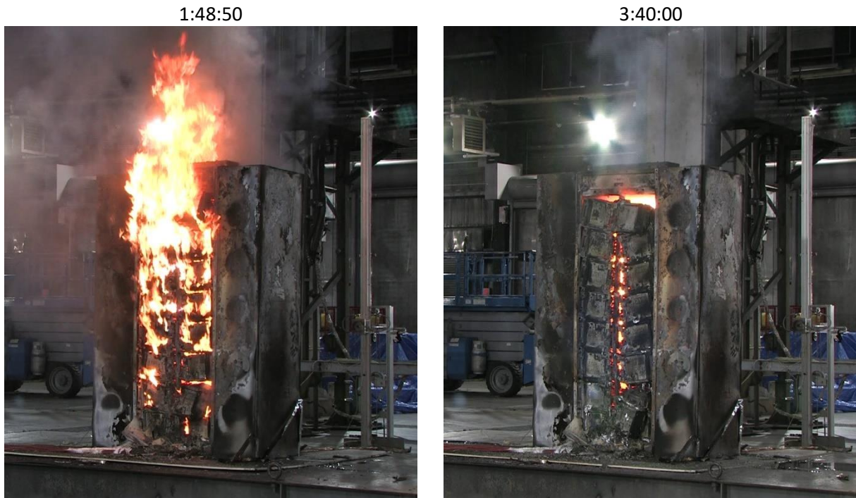
Figure 6-6: Photos of NMC fire decay phase before firefighter intervention (fire did not self-extinguish). Notice the furnace type combustion evident as the combustion transition to within the rack.
