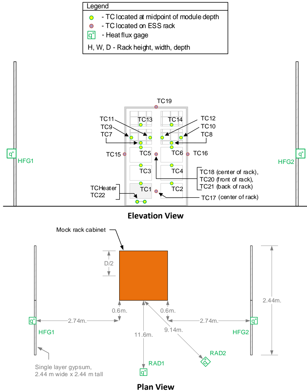
Figure 5-2: Schematics of intermediate-scale free burn fire test and instrumentation layout (not to scale) for NMC test. Front elevation view shown on top and plan view on bottom. Checkered boxes in elevation view represent the location of 'mock' modules.
