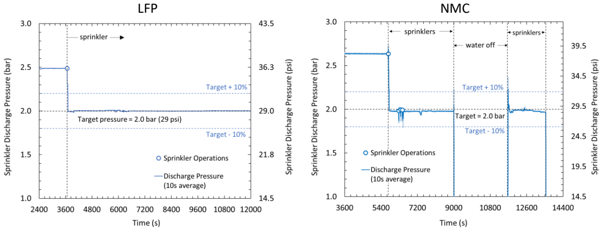
Figure 6-32: Sprinkler discharge pressure during LFP (left) and NMC (right) tests.
