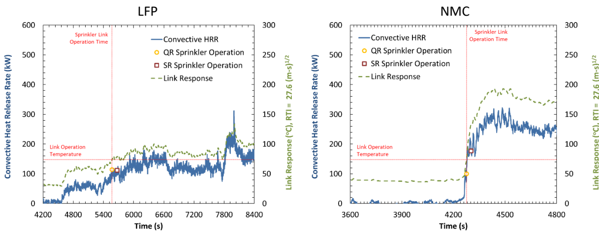
Figure 5-10: Predicted sprinkler response during LFP (left) and NMC (right) free burn test. Dashed green line shows the response of a QR link installed under a 4.6 m (15 ft) ceiling, directly over the fire.
