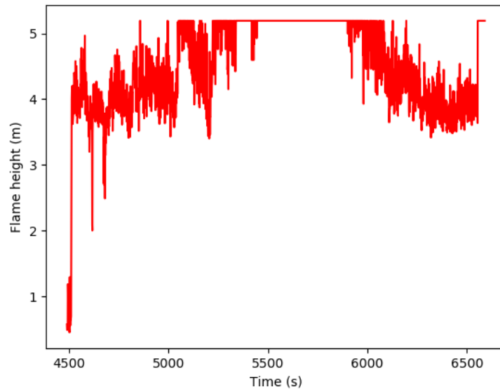
Figure A-5: Flame heights of NMC fire test.
