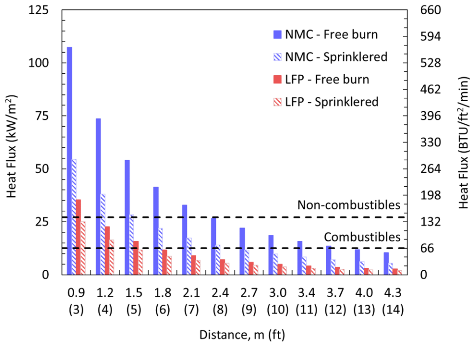
Figure 7-2: Predicted thermal exposure to combustible and non-combustible objects as a function of distance. Results are based on large-scale testing of an 83 kWh LFP system and 125 kWh NMC system.
