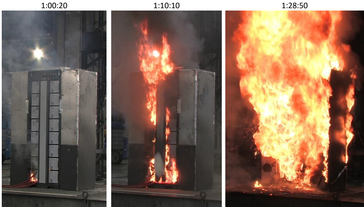
Figure 6-5: Photos of NMC fire development during large-scale free burn test: near time of ignition (left), near time of predicted sprinkler operation (middle), peak heat release rate (right).
