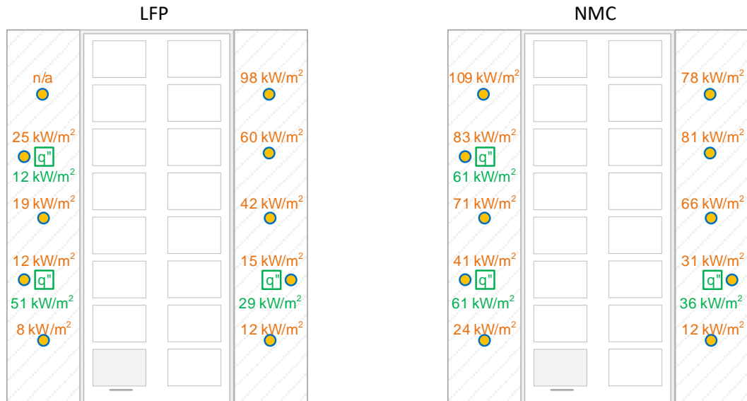
Figure 6-14: Peak instantaneous thermal exposure to adjacent ESS racks from LFP (left) and NMC (right) tests.
