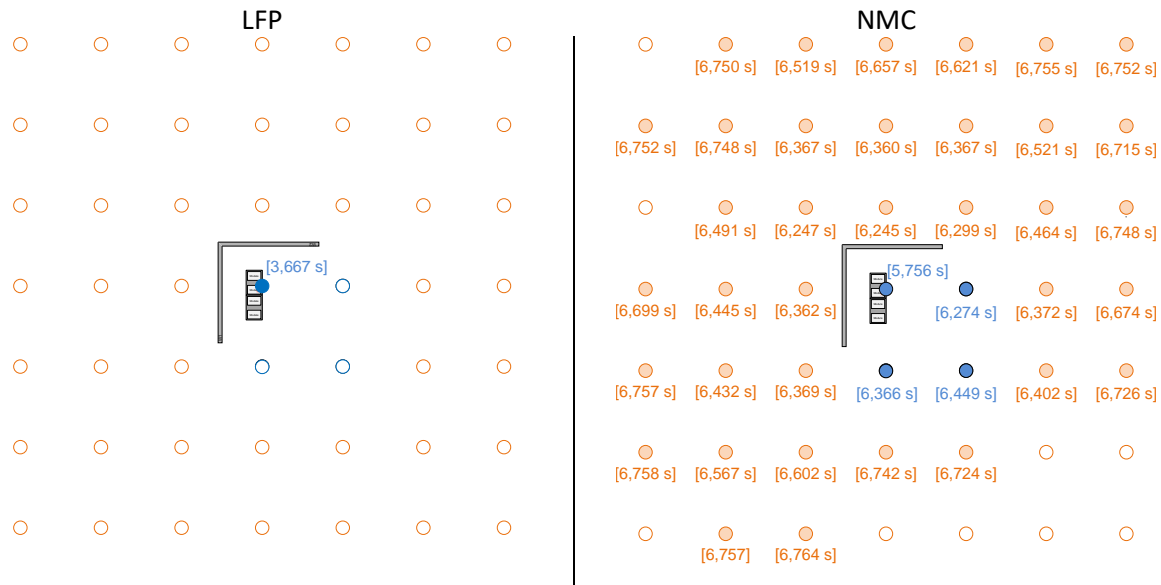
Figure 6-29: Sprinkler operation overview for LFP (left) and NMC (right) tests. Sprinklers that operated are shown as solid circles. Blue circles represent active sprinklers that could discharge water and orange circles represent indicator sprinklers that could not.
