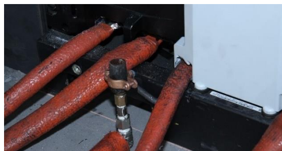
Figure 4-5: Supplemental pilot flame used to ensure ignition of vent gases for the LFP modules.
