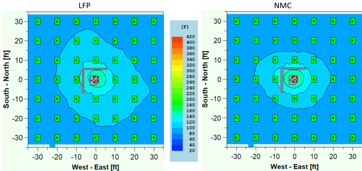
Figure 6-30: Contour plots of ceiling gas temperatures at first sprinkler operation during LFP (left) and NMC (right) tests. Convert to metric as [m = ft \times 0.305] and [^{\circ}C = (^{\circ}F - 32)/1.8] .
