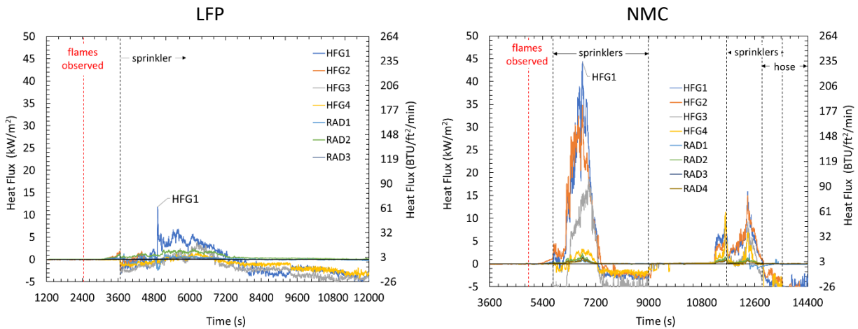
Figure 6-27: Thermal exposure to surrounding objects during LFP (left) NMC (right) during test.
