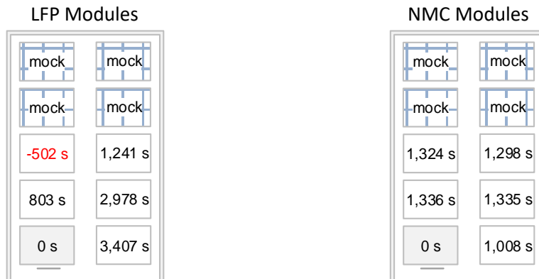
Figure 6-9: Module temperature exceedance time of 150°F (66°C) during large-scale tests. Time shown from first observation of flames on ignition module.
