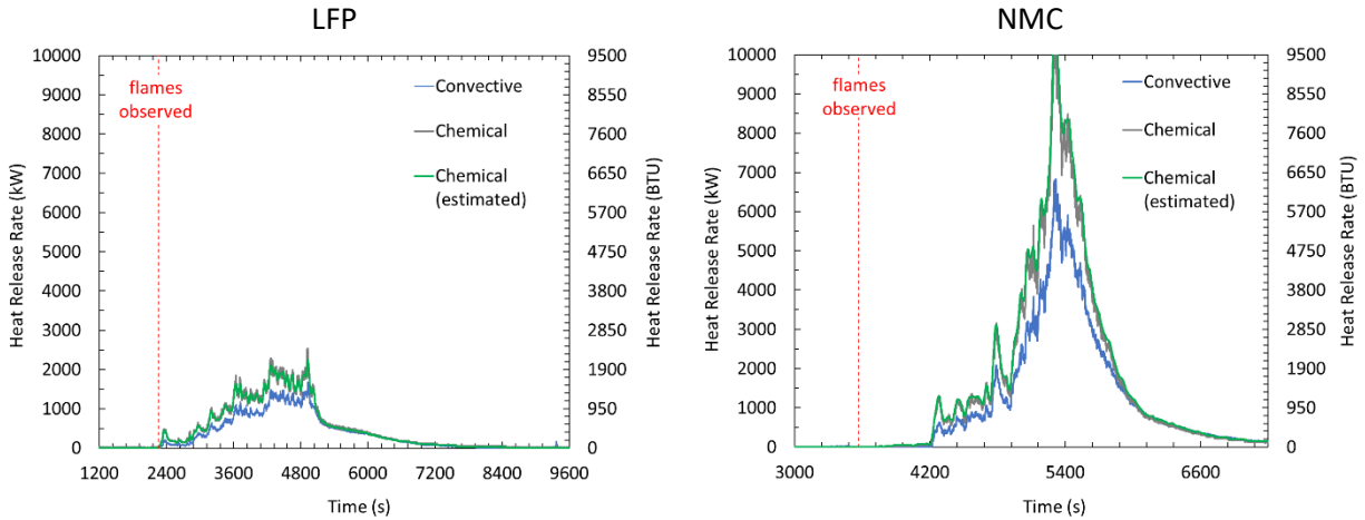
Figure 6-15: Heat release rate for LFP (left) and NMC (right).
