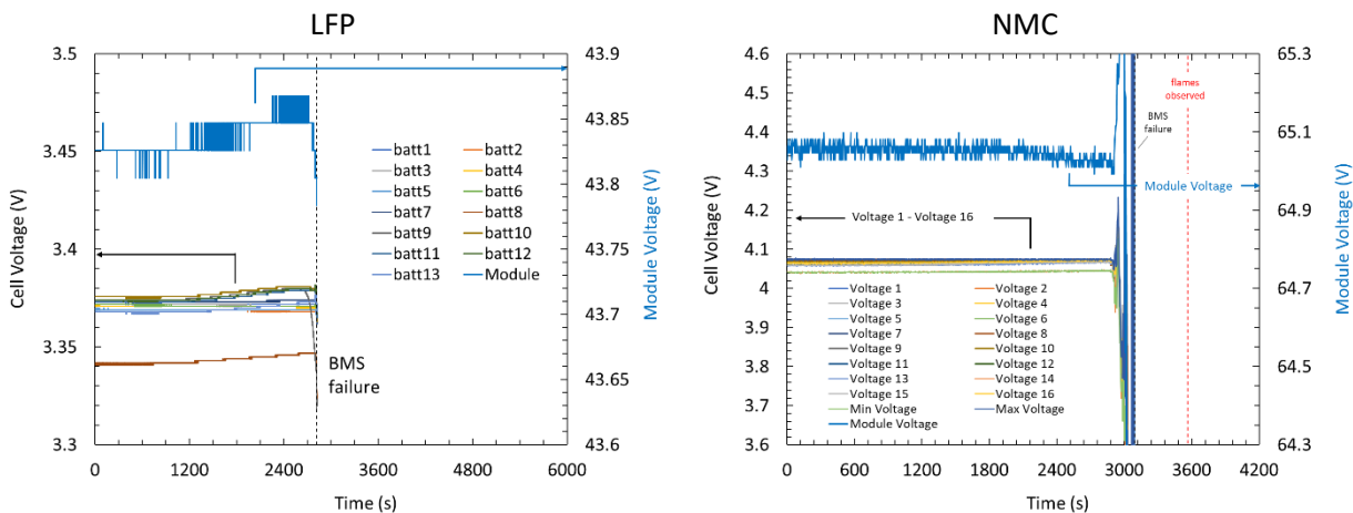
Figure D-1: Voltage measurements from module BMS for LFP (left) and NMC (right) tests.
