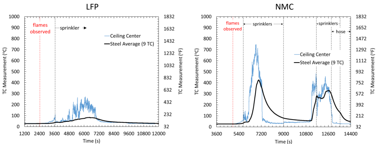
Figure 6-31: Ceiling steel TC measurements and gas temperature at the ceiling center during LFP (left) and NMC (right) test.
