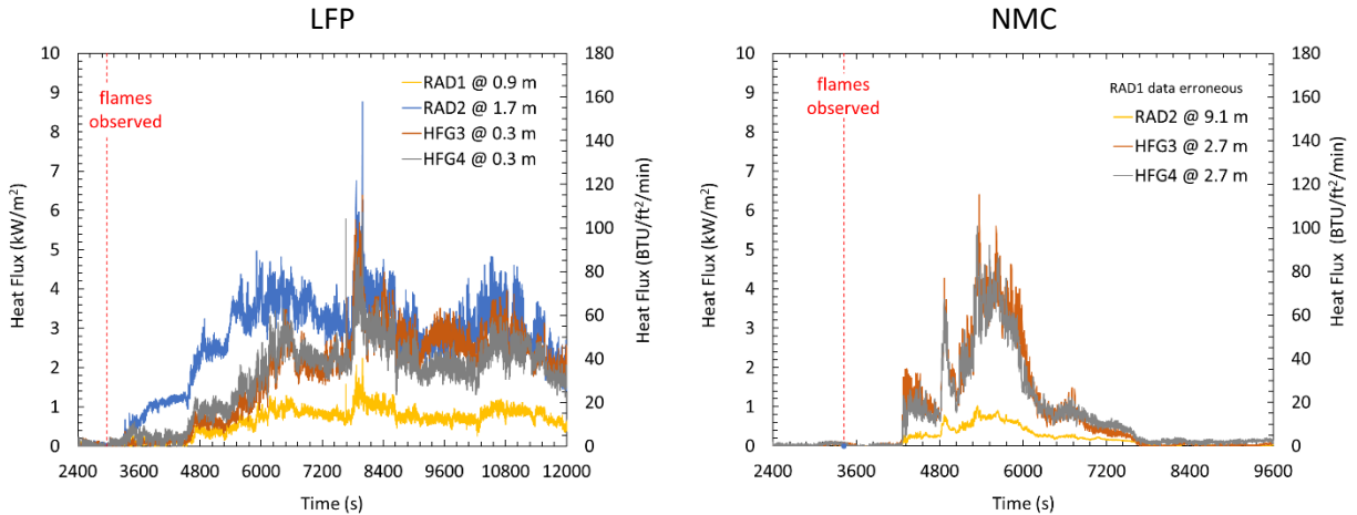
Figure 5-8: Thermal exposure to surroundings during LFP (left) and NMC (right) test.
