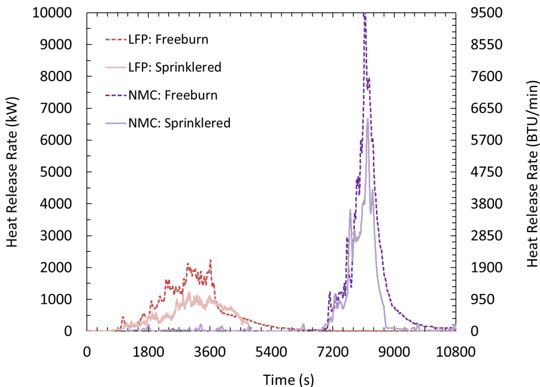
Figure 7-1: Comparison of heat release rate during free burn and sprinklered tests. Times are offset to group LFP and NMC data.
