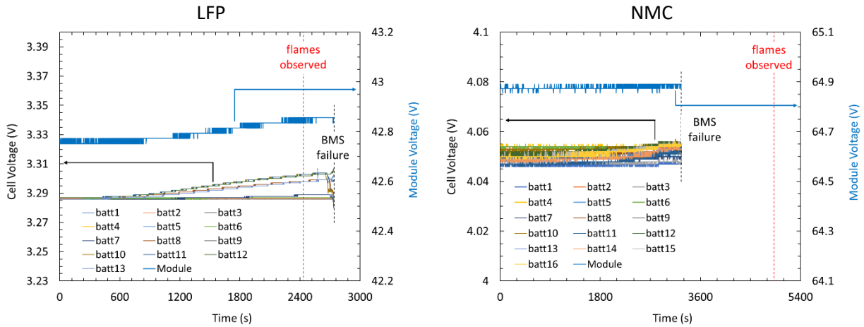
Figure D-3: Voltage measurements from module BMS for LFP (left) and NMC (right) tests.
