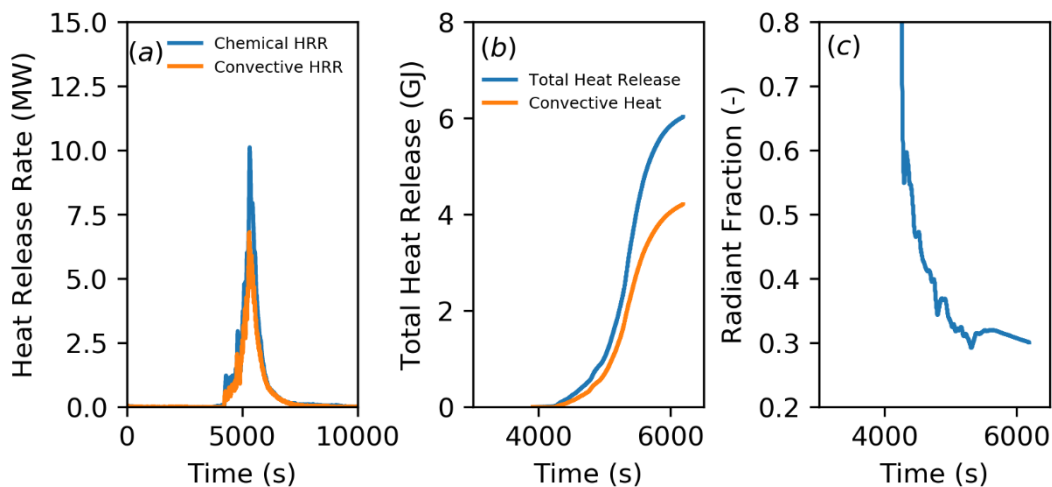
Figure A-4: NMC free-burn fire test (a) Chemical and convective heat release rates; (b) total chemical heat release and convective heat release; (c) radiant fraction.
